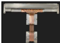
Two CPU solution : Total 1000W Heat pipe length > 600mm
